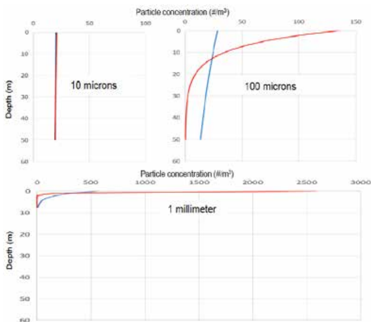
Figure 5.1 Modelled vertical distribution of particles in the upper ocean with a constant surface wind of 7 \text{ m s}^{-1} , for three size categories (10 \mu\text{m} , 100 \mu\text{m} and 1 mm) and two buoyant polymer types of differing density and hence buoyancy: red – polybutylene ( \rho = 0.60 \text{ cm}^{-3} ) and polyethylene HDPE ( \rho = 0.97 \text{ cm}^{-3} ), (Sven Sundby unpublished).
